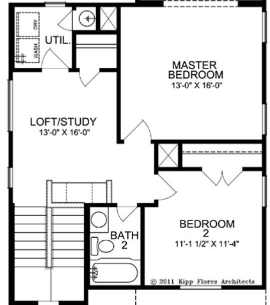
OPTIONAL 2ND FLOOR PLAN W/ OPTIONAL GARAGE AT 1ST FLOOR
