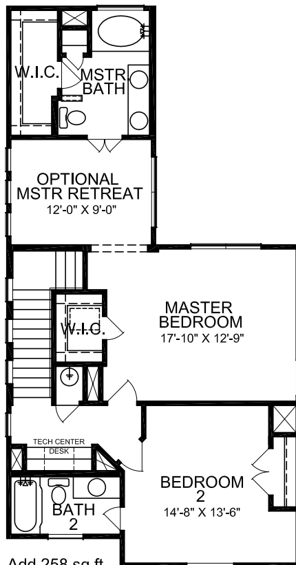
Add 258 sq ft OPTIONAL SECOND FLOOR 1
